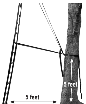
Figure 27 Treestand Set Correctly
