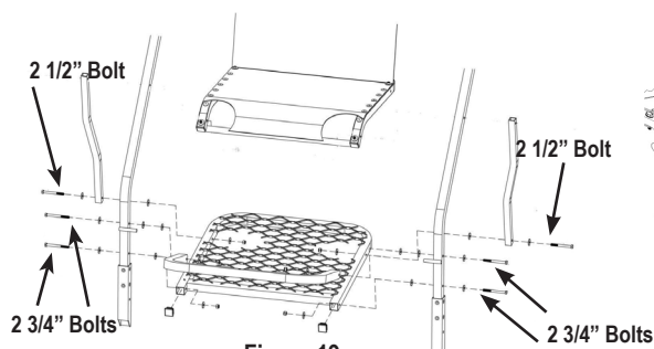
Figure 19 Install Platform and Platform Support Braces
