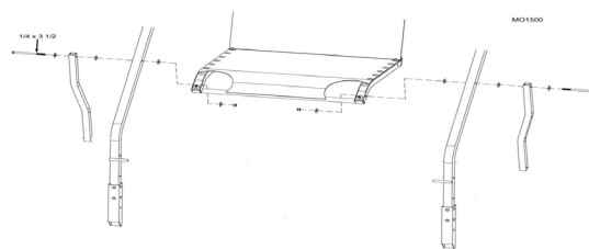
Figure 18 Install Seat Platform and Platform Support Braces Onto Uprights
