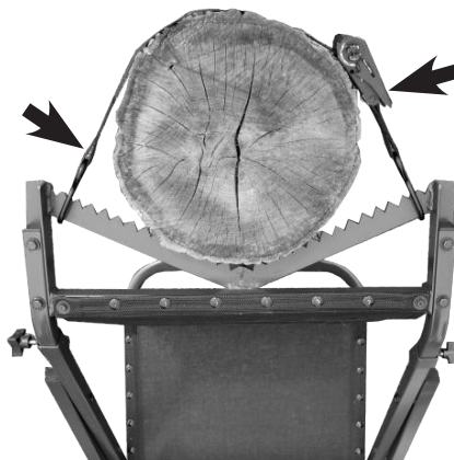
Figure 34 Ratchet Strap Attached to Tree Trunk (Cutaway tree view)
