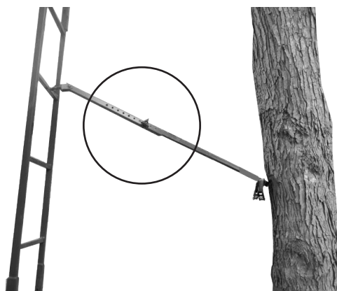
Figure 28 Tree Brace Placed
