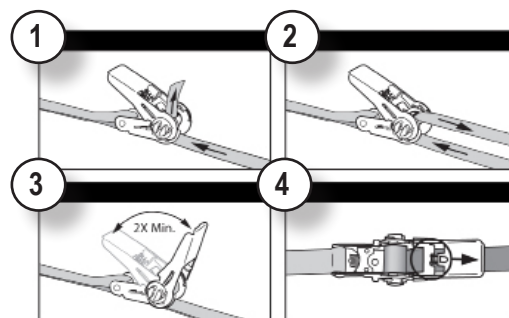
Figure 35 Ratchet Threading
