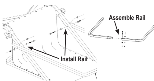
Figure 20 Assemble/Install Shooting Rail
