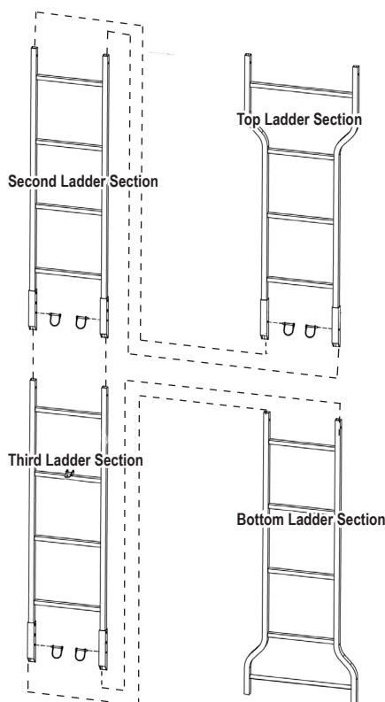
Figure 22 Connect Ladder Sections Using Spring Pins
