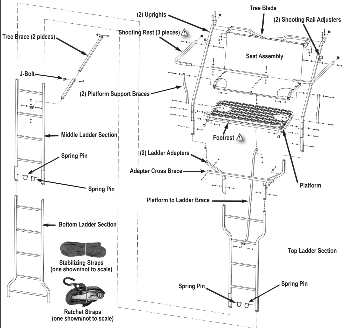
Figure 15 Components of the L200 18' Double Ladderstand
