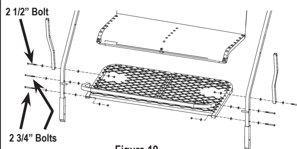
Figure 19 Install Platform and Platform Support Braces
