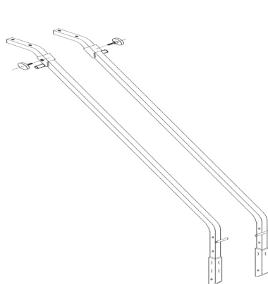
Figure 16 Install Shooting Rail Adjusters on Uprights
