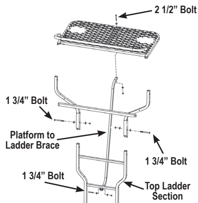
Figure 24 Install Platform to Ladder Brace
