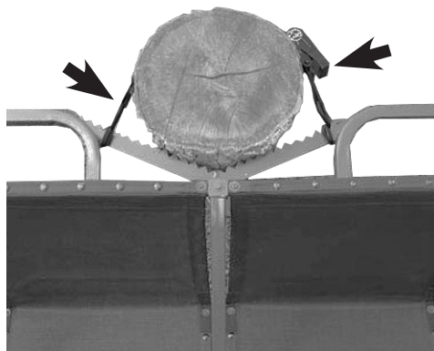
Figure 37 Ratchet Strap Attached to Tree Trunk (Cutaway tree view)
