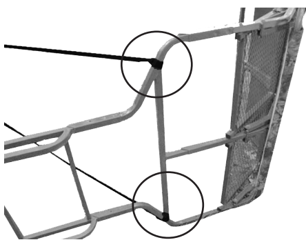
Figure 27 Secure the Stabilizing Straps to Ladder Adapters
