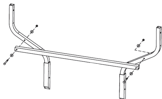
Figure 22 Assemble Ladder Adapters and Adapter Cross Brace
