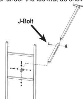
Figure 21 Connect Tree Brace to Middle Ladder Section
