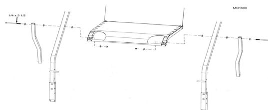
Figure 18 Install Seat Platform and Platform Support Braces Onto Uprights
