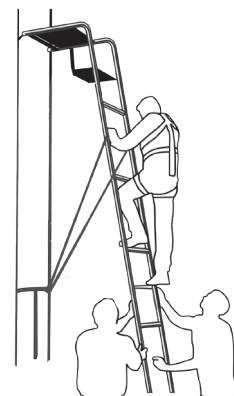
Figure 35 Two Adults to Help Steady Treestand Assembly (Representative ladder-stand shown)
