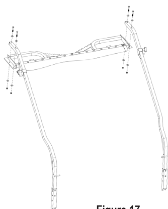
Figure 17 Install Tree Blade Assembly Onto Uprights
