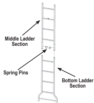
Figure 25 Connect Middle and Bottom Ladder Sections (Tree Brace Not Shown for Clarity)
