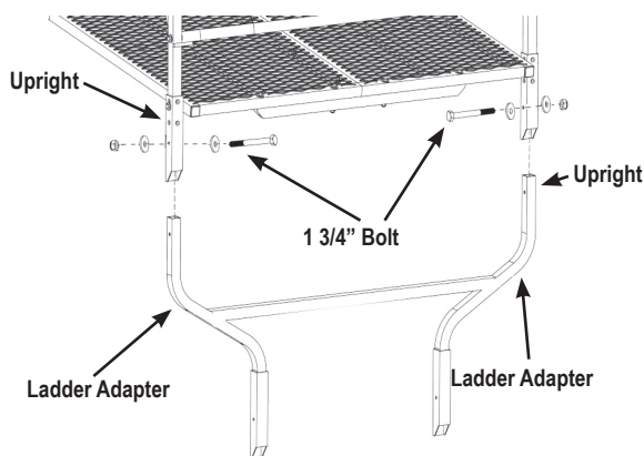
Figure 23 Install Ladder Adapters to Uprights
