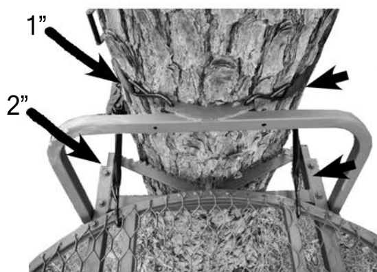
Figure 37 Ratchet Straps Attached to Tree Trunk
