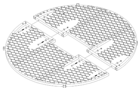
Figure 16 Assemble Standing Platform
