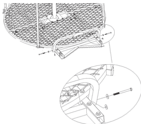
Figure 22 Install Second Tree blade
