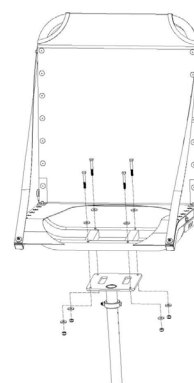
Figure 25 Install the Seat on the Seat Post
