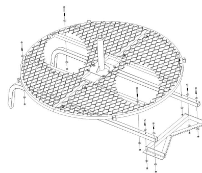
Figure 18 Attach Tree Blade to Horizontal Support Tubes and Standing Platform to Support Tubes
