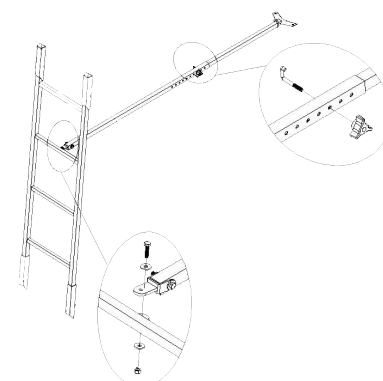
Figure 21 Install Tree Brace
