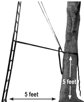
Figure 30 Treestand Set Correctly
