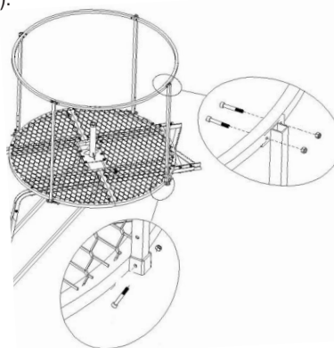
Figure 20 Install Shooting Rail
