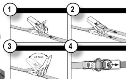
Figure 38 Ratchet Threading
