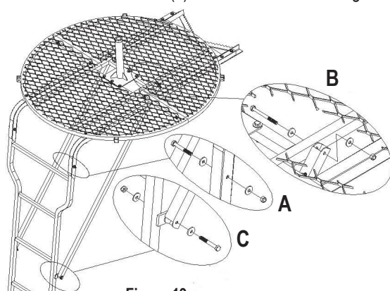
Figure 19 Attach Top Ladder Section and Diagonal Supports
