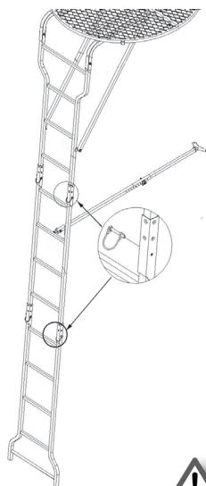
Figure 23 Assemble Ladder Sections
