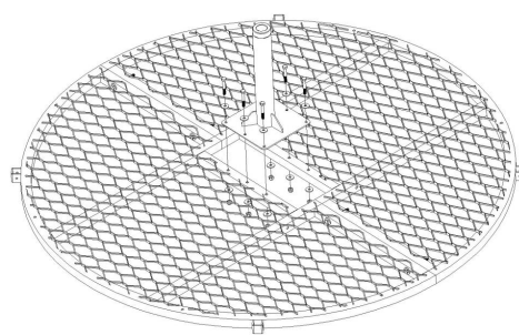
Figure 17 Install Seat Base onto Standing Platform
