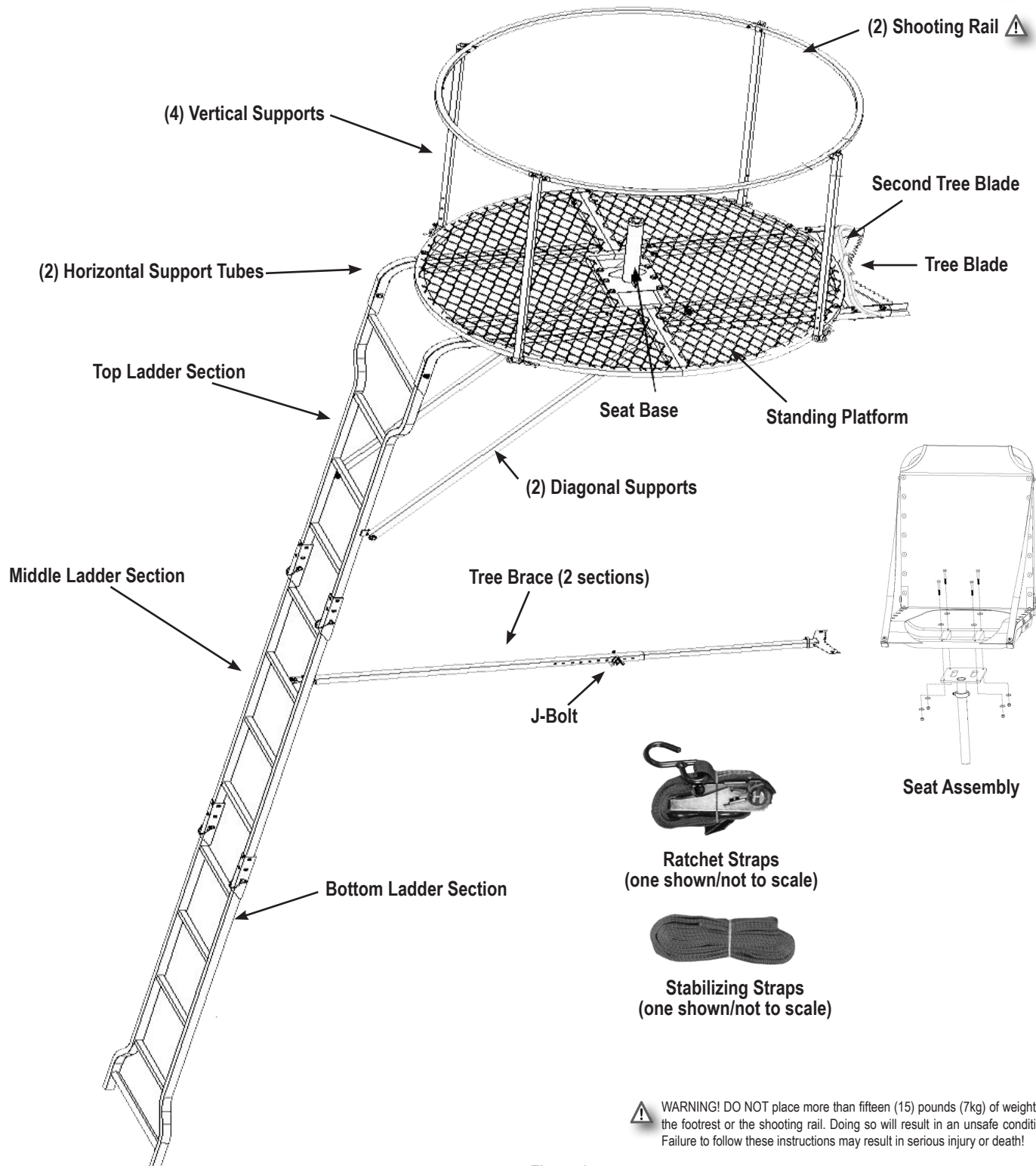
Figure 15 Components of the L360 Ladderstand
