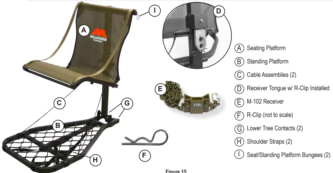
Figure 15 Components of the Millennium M-100U w/ M-102 Receiver
