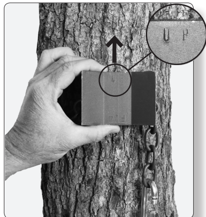
Figure 3 M-102 Receiver Positioned Upward
