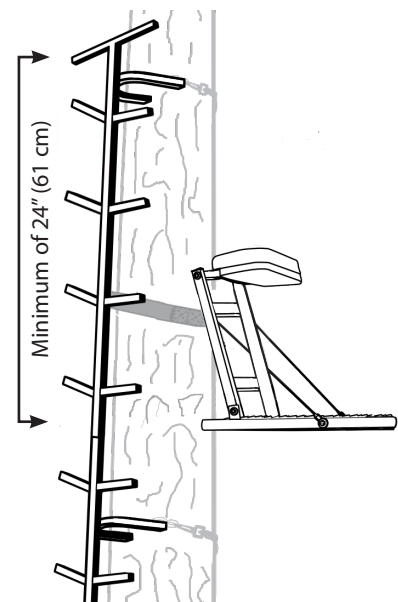
Figure 8 Climbing system installed a minimum of 24" above standing platform
