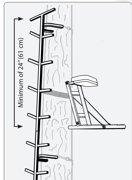
Figure 1 Climbing system installed a minimum of 24" above standing platform
