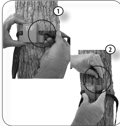
Figure 10 Insert Loop End Into Receiver
