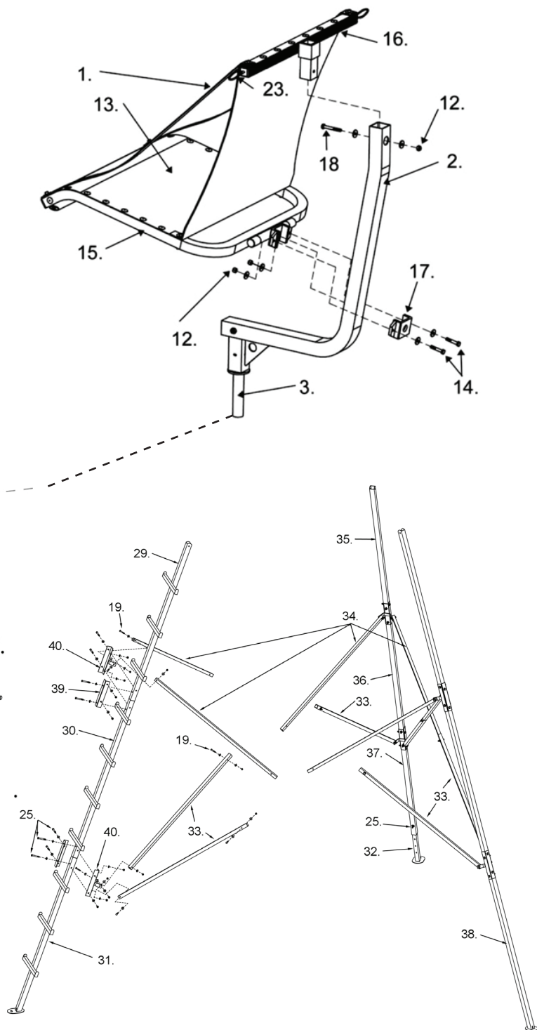
Figure 15 Components of the T-360 Tripod
