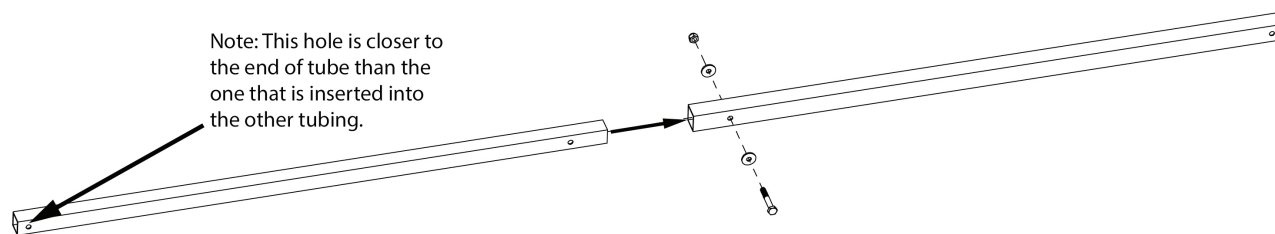
Figure 22 Assemble Cross Braces
