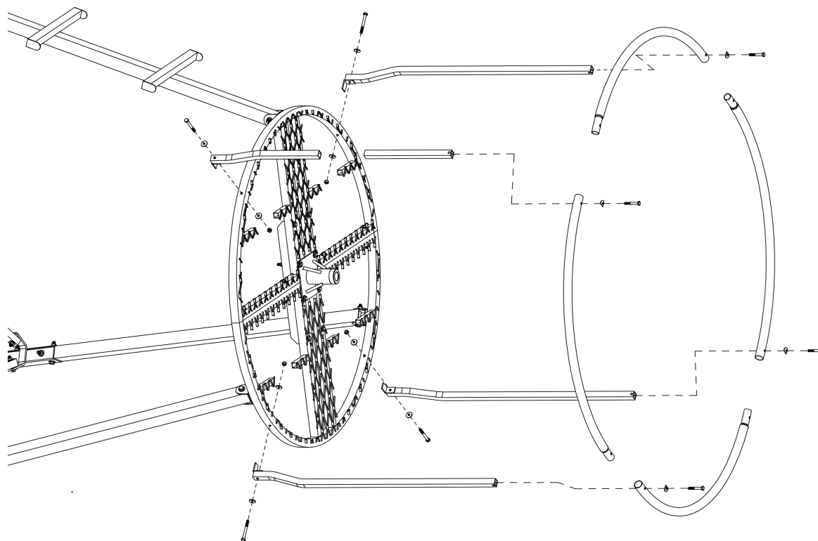
Figure 28 Attach Shooting Rail
