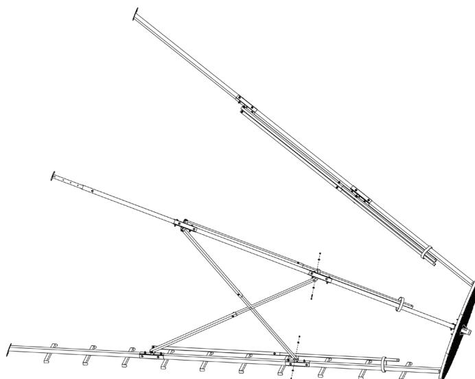
Figure 27 Attach Cross Braces
