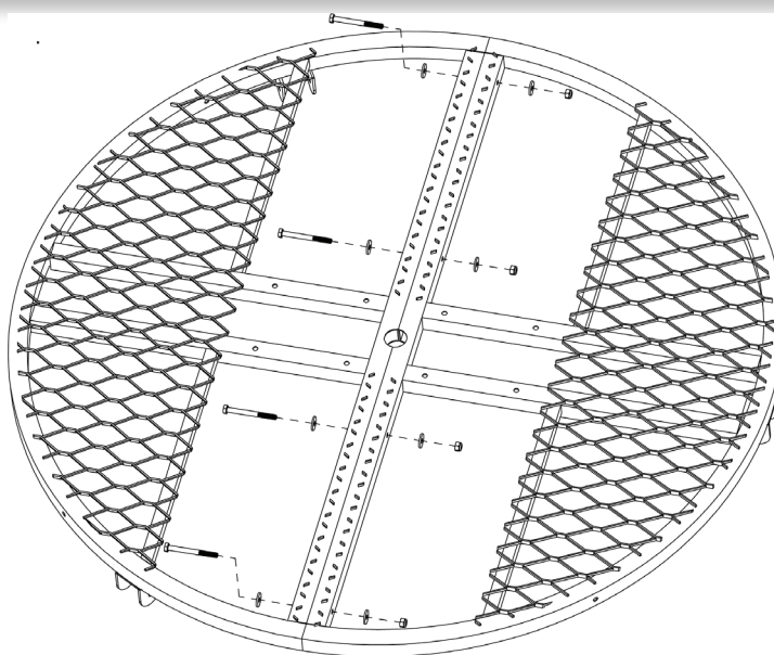
Figure 17 Bolt Platform Together
