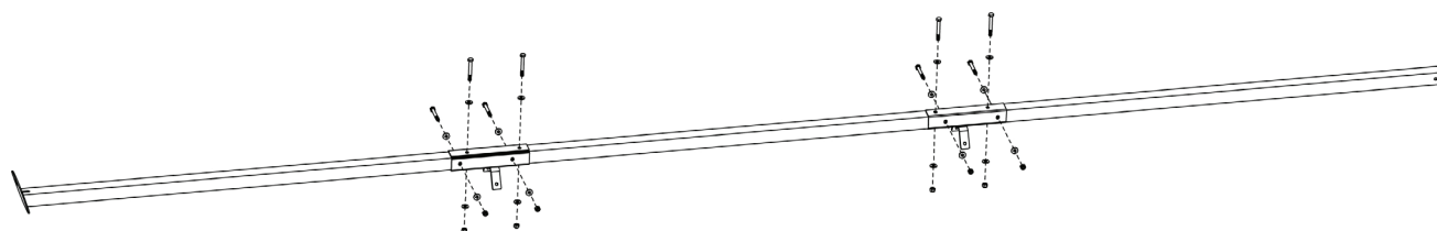
Figure 19 Assemble Three Ladder Sections
