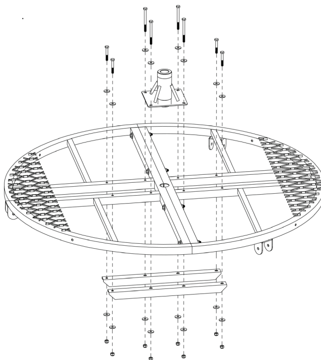
Figure 18 Install Seat Receiver
