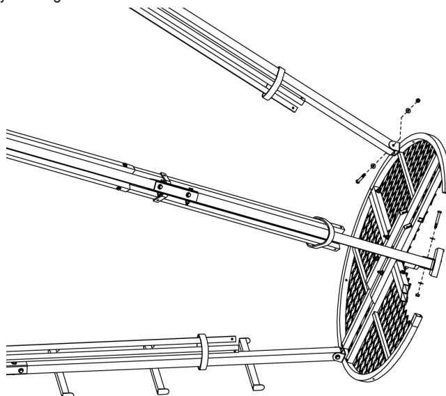
Figure 26 Attach Remaining Legs
