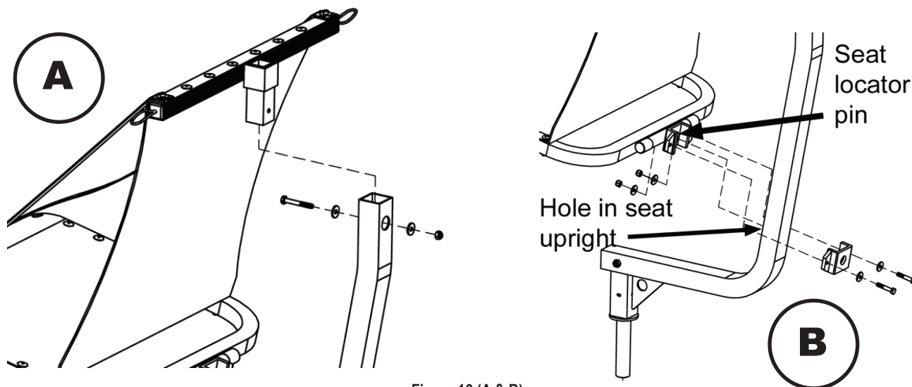
Figure 16 (A & B) Seat Assembly
