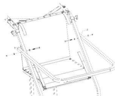
Figure 24 Install Shooting Rail
