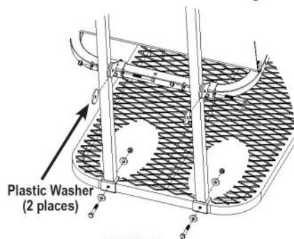
Figure 22 Seat Hinge Disc Orientation
