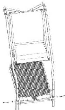
Figure 19 Install Platform Onto Uprights
