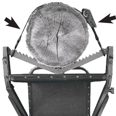
Figure 37 Ratchet Strap Attached to Tree Trunk (Cutaway tree view)
