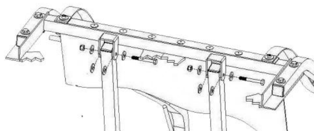
Figure 20 Install Vertical Supports (Tree Blade Cutaway for Clarity)
