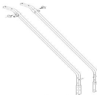
Figure 17 Install Shooting Rail Adjusters
