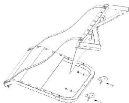
Figure 16 Install Hinges
