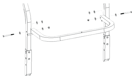
Figure 25 Install Foot Rest
