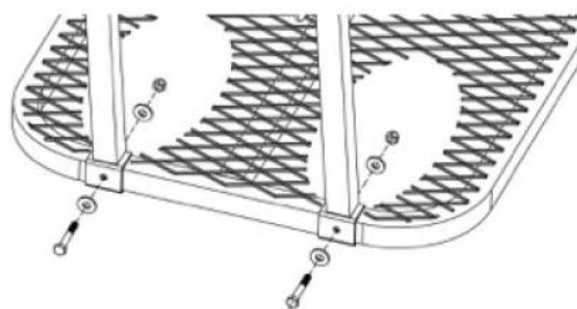
Figure 23 Install Vertical Supports to Platform
