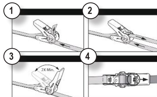
Figure 38 Ratchet Threading
