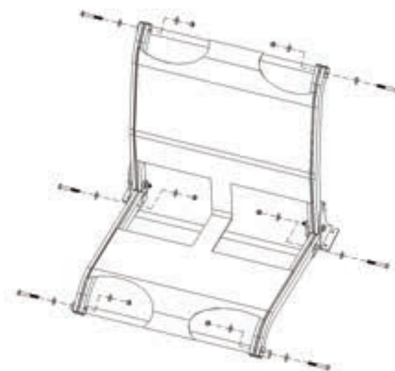
Figure 23 Install the Seat Spreader Bars
