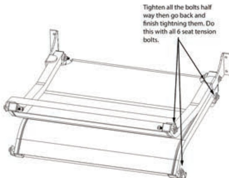
Figure 25 Tighten Seat Tension Bolts
