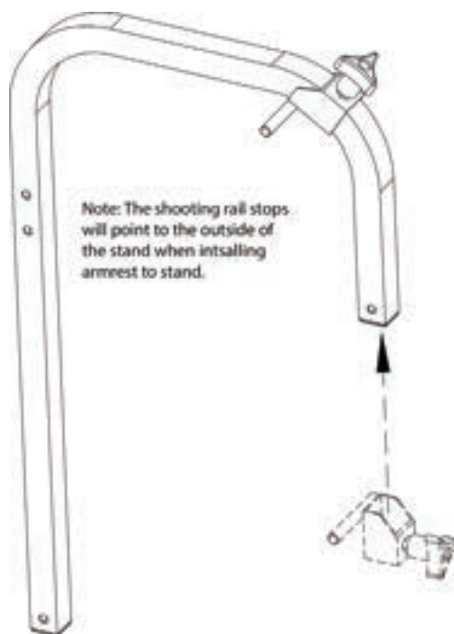
Figure 18 Install Shooting Rail Adjusters on Arm Rest
