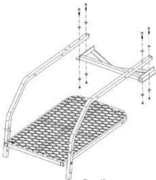
Figure 17 Install Tree Blade Assembly
