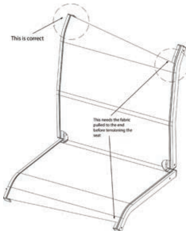
Figure 24 Pull Seat Fabric to End of Seat Frame
