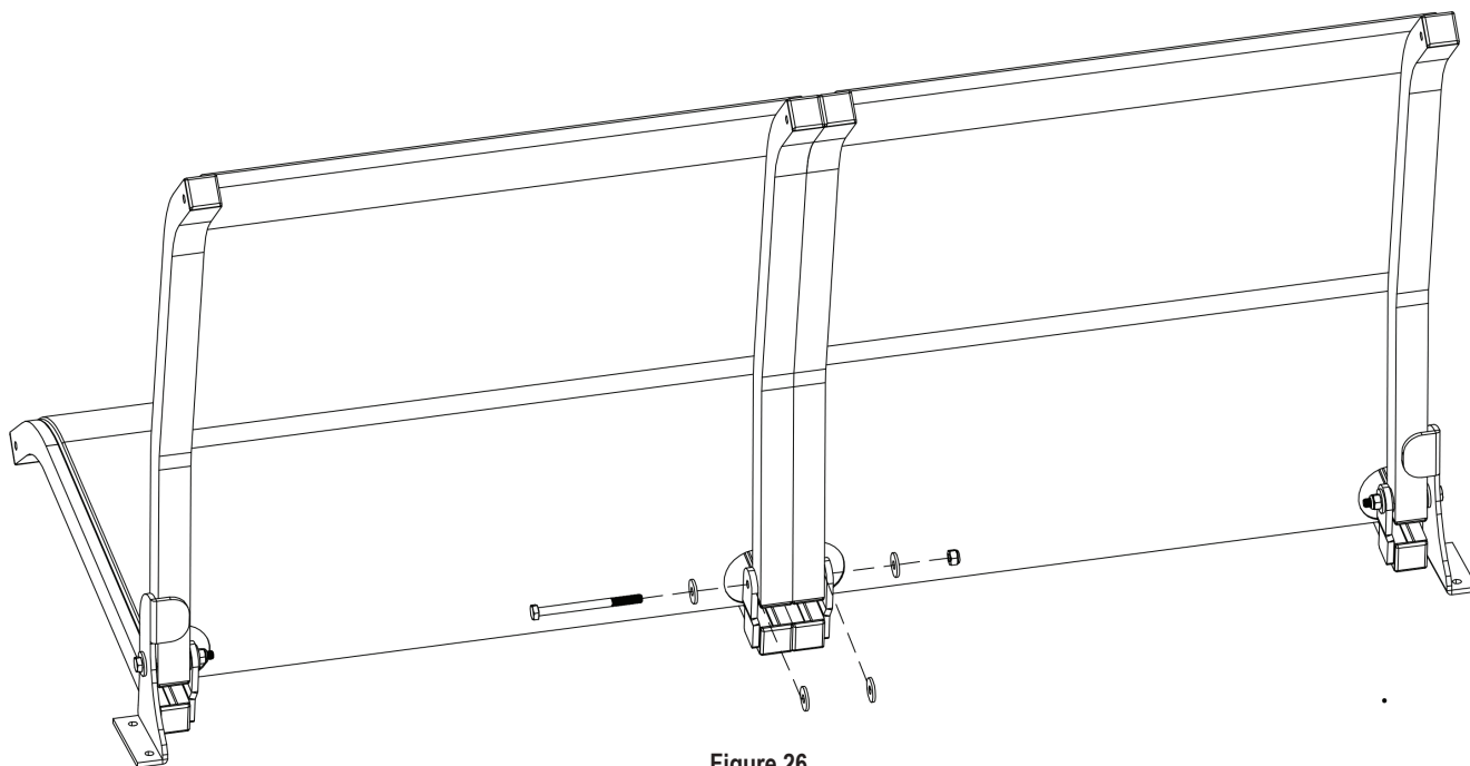
Figure 26 Seat Assembly
