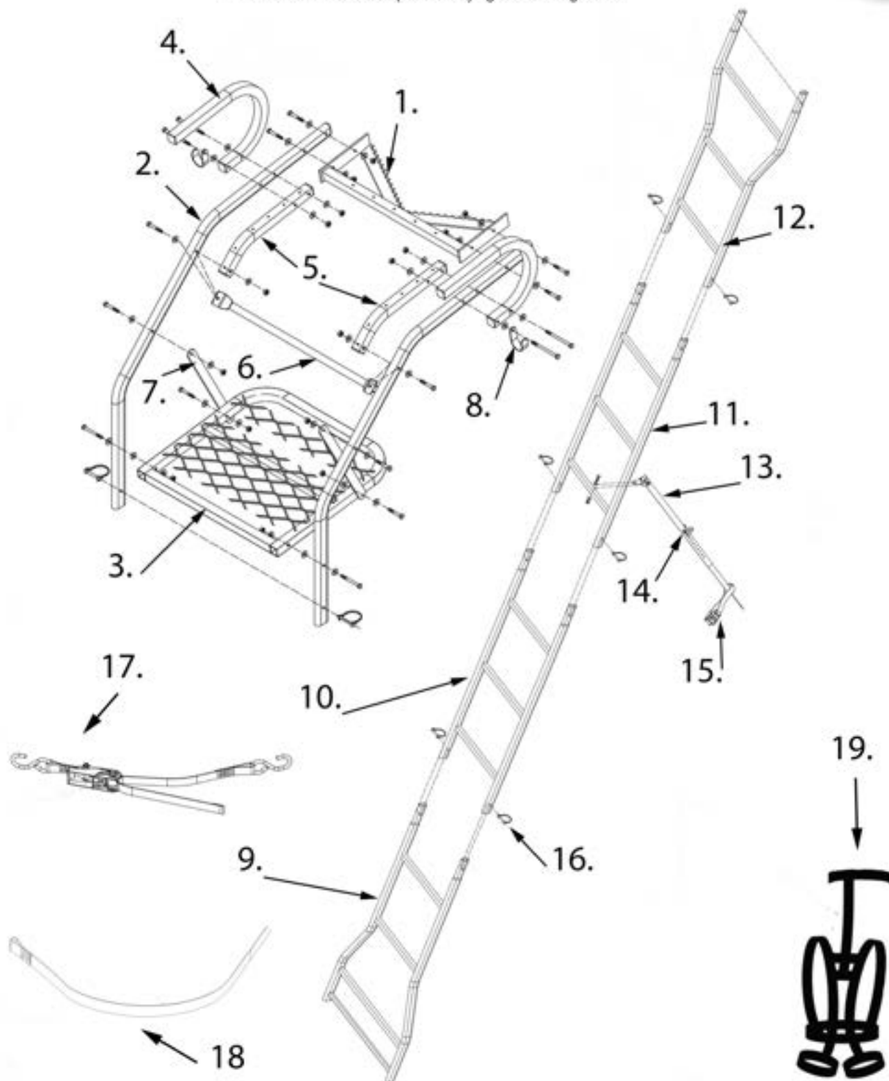
Figure 15 Components of the L-118 Ladderstand
