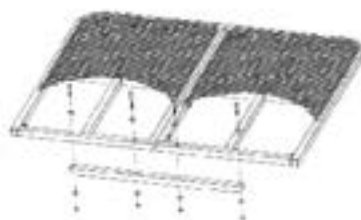
Figure 17 Install Platform Reinforcement Tube to Platform
