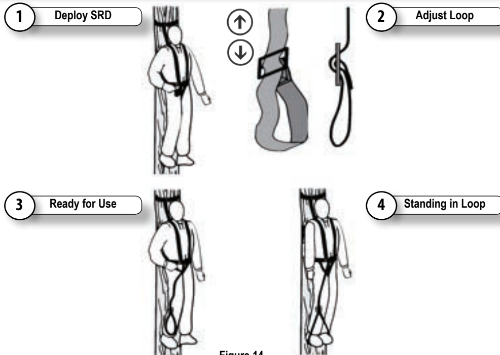
Figure 14 Suspension Relief Device (SRD) Operation
