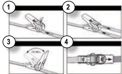
Figure 36 Ratchet Threading
